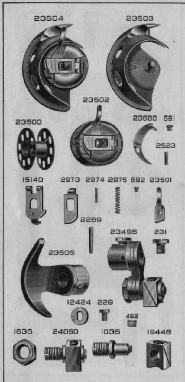
PLATE 4017—FULL SIZE
