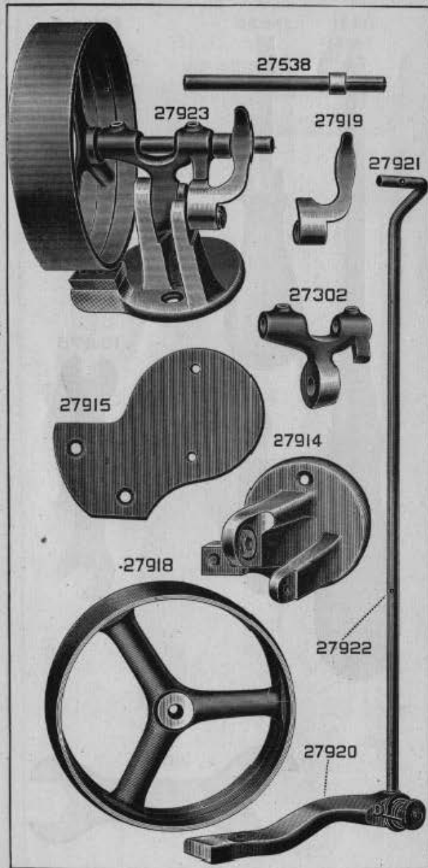
PLATE 4029 - ONE-HALF SIZE
