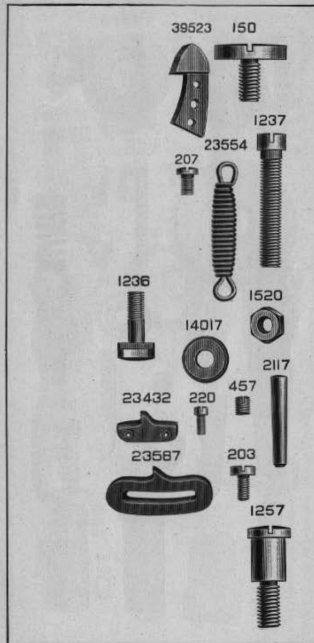
PLATE 4012—FULL SIZE
