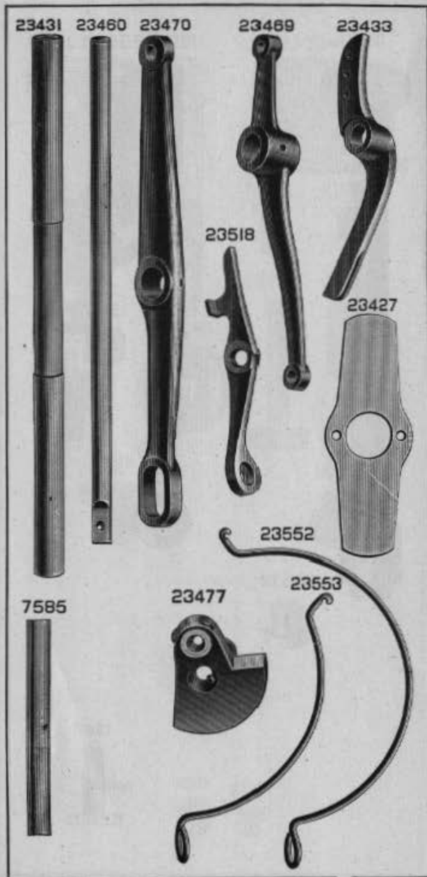
PLATE 4010—ONE-HALF SIZE
