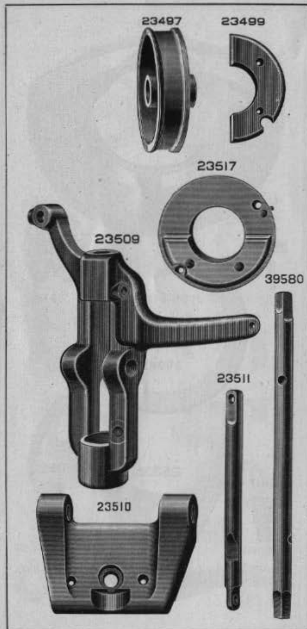
PLATE 4019—ONE-HALF SIZE
