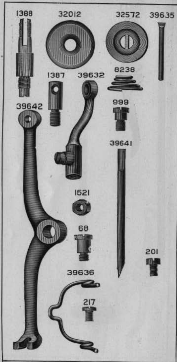
PLATE 4052—FULL SIZE
