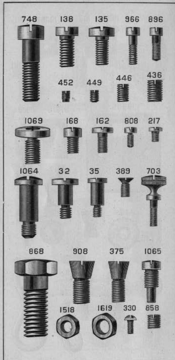
PLATE 4025—FULL SIZE
