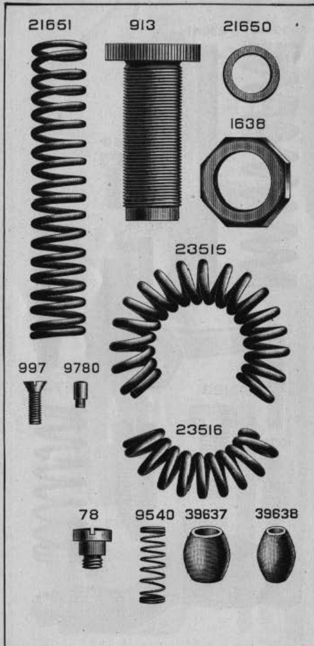
PLATE 4021—FULL SIZE
