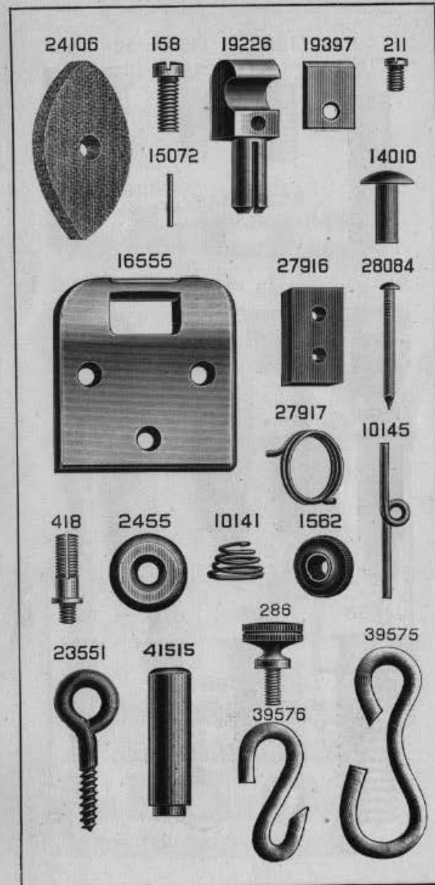
PLATE 4024—FULL SIZE
