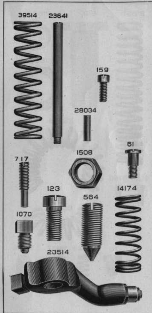
PLATE 4020—FULL SIZE
